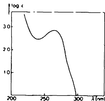
Fig. 4 UV-spectrum of I_c in iso-octane.
