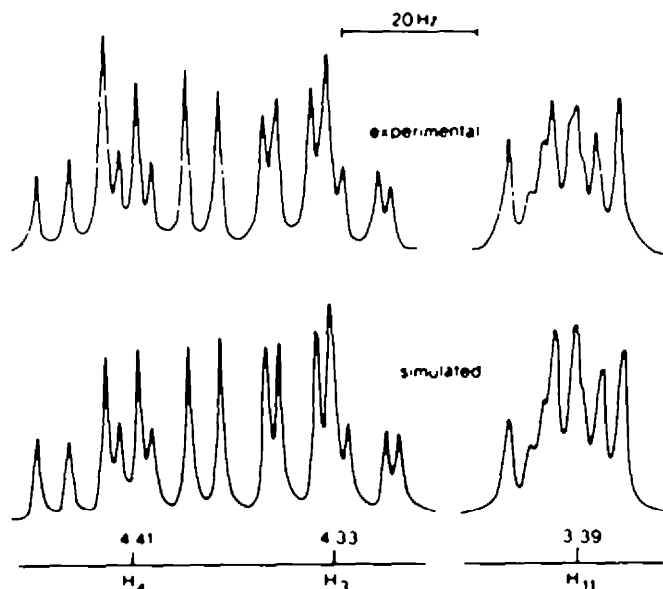
Fig. 3. ^1\text{H-NMR} signals of protons \text{H}_3 , \text{H}_4 and \text{H}_{11} , simulated and experimentally obtained on a 360 MHz apparatus.
