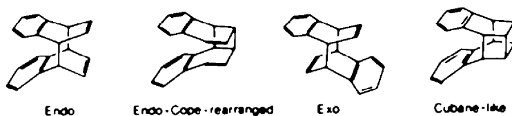
Fig. 1 Structure of dimers of naphthalene derivatives
